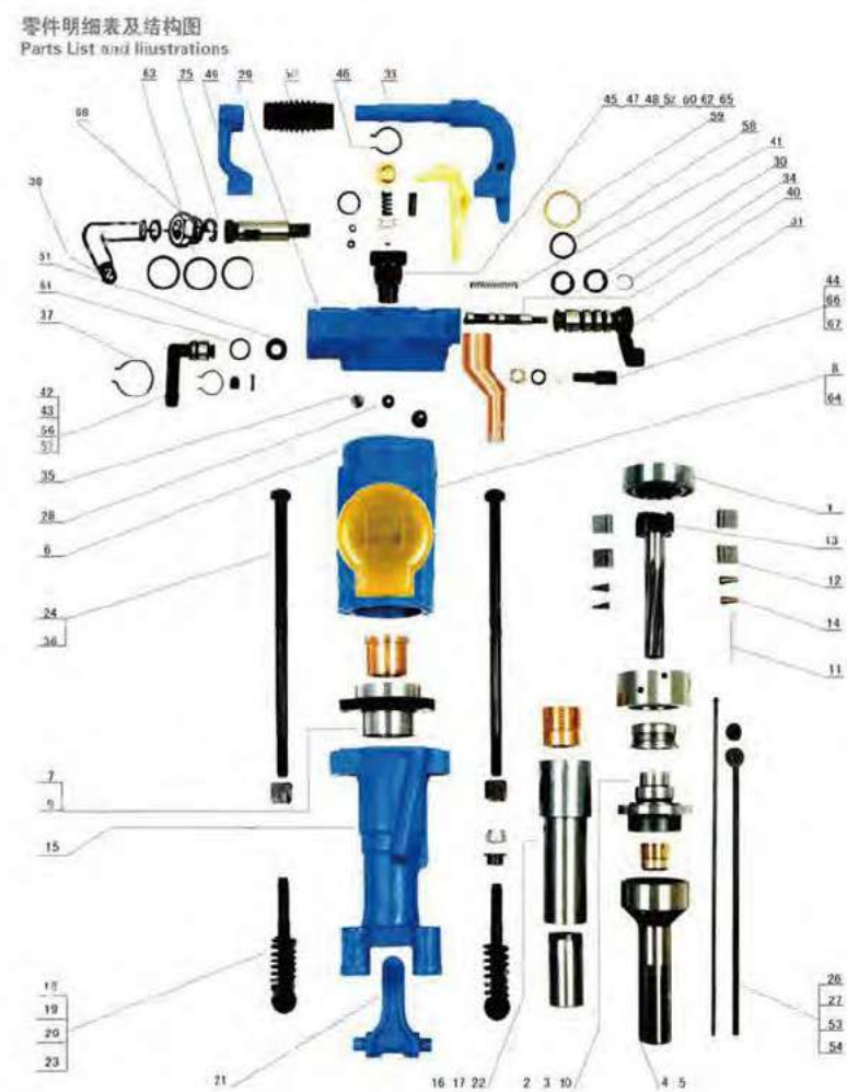
[ YT28型凿岩机分解图 ] YT28 SLB0 ILLUSTRATION
